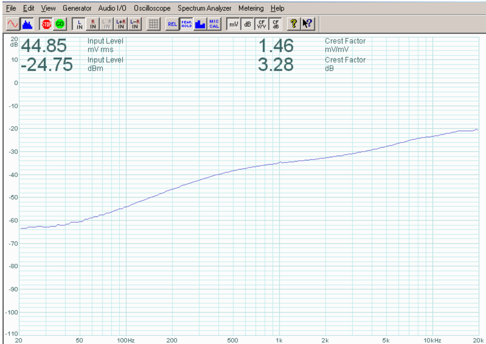
Inverse-RIAA Equalization Curve Input signal: Sine wave sweep, 20 to 20,000 Hz at 0dB
